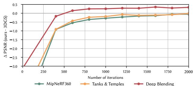
Fig. 11. Finetuning Pretrained 3DGS Models : After only 500 iterations of finetuning, we can recover most of the perceptual quality of 3DGS [Kerbl et al. 2023]. After 2k iterations we match or outperform 3DGS across all datasets.
