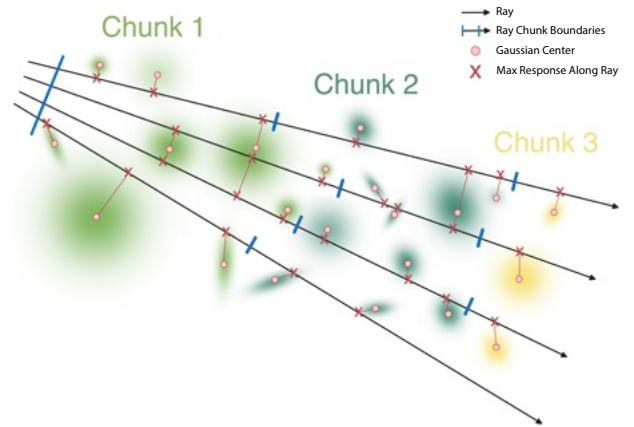
Fig. 5. Rendering: on each round of tracing, the next k closest hit particles are collected and sorted into depth order along the ray, the radiance is computed in-order, and the ray is cast again to process the next chunk.
