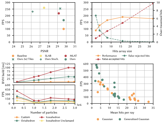
Fig. 8. Quantitative Ablation. Top left: comparison of the different tracing algorithms on the combination of our datasets. Top right: Impact of the hit payload buffer size on our proposed tracing algorithm. Bottom left: Impact of the different primitives on both the BVH building time and the FPS. Bottom right: Mean number of hits vs. mean FPS for every sequence of our dataset.
