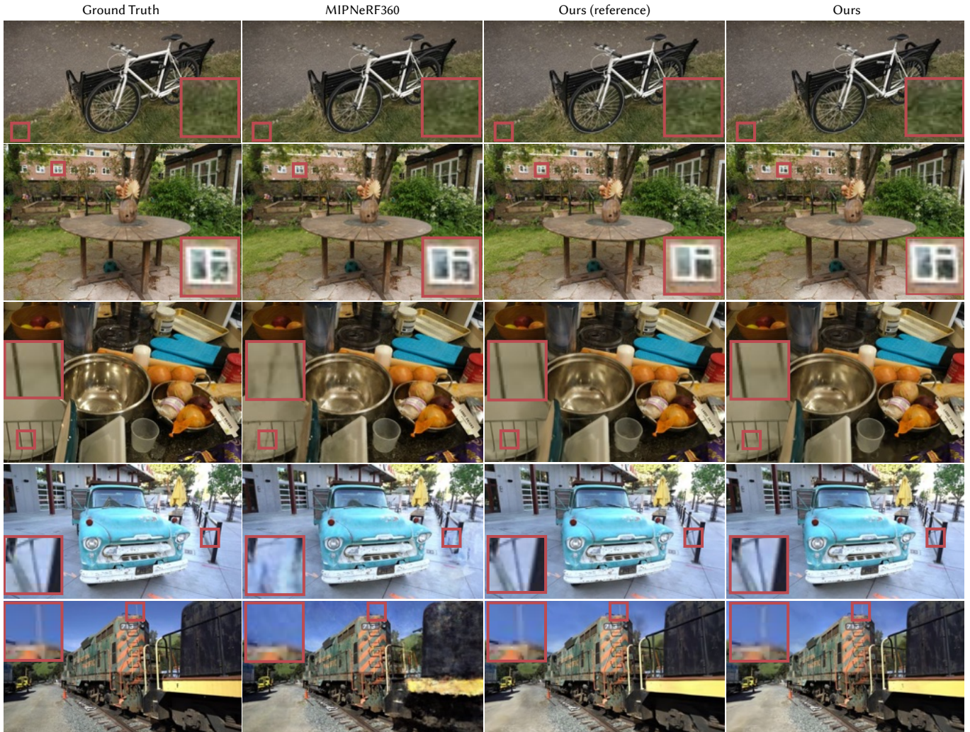
Fig. 17. Additional Qualitative Comparisons: novel-view synthesis results relative to the MIPNeRF360 baseline (insets (●) show per-result closeups).
