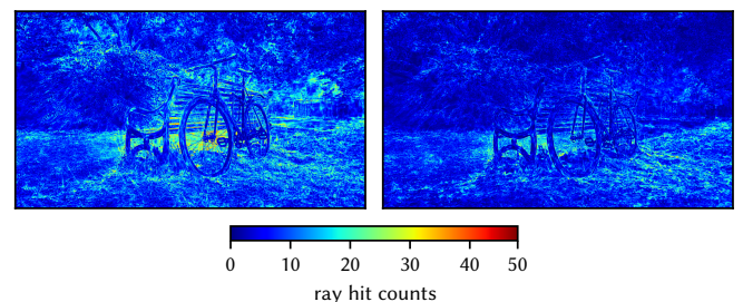
Fig. 9. Ray Hits for Kernel Functions: Visualization of the number of per-ray particles hits for the Gaussian (left) and for the generalized Gaussian kernel function of degree 2 (right) (• represents no hits).
