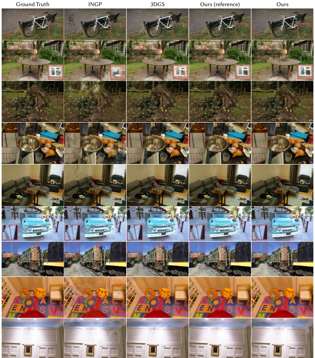
Fig. 7. Novel-View Synthesis: Qualitative comparison of our novel-view synthesis results relative to baselines (insets (•) show per-result closeups). For fairness, this comparison uses the same test views picked by [Kerbl et al. 2023]. Additional comparisons with [Barron et al. 2022] are included in the appendix.
